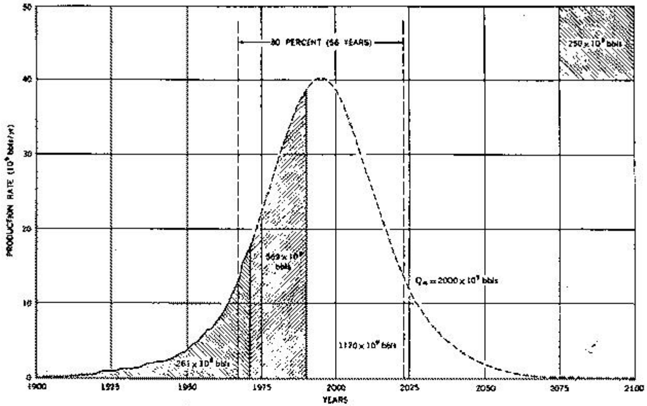
Fig. 8 - Complete-cycle curve for world crude-oil production (Hubbert, 1974a, fig. BB).
