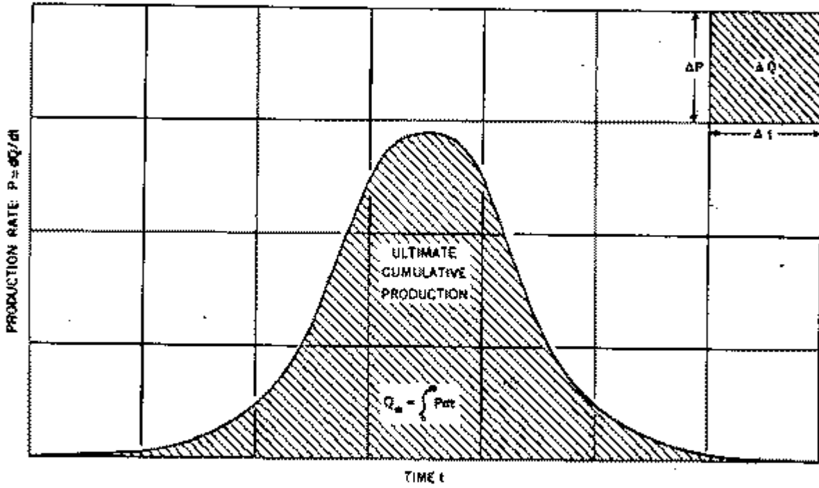
Fig. 6 - Mathematical properties of complete-cycle curve of production of exhaustible resource (Hubbert, 1974a, fig. 18).
