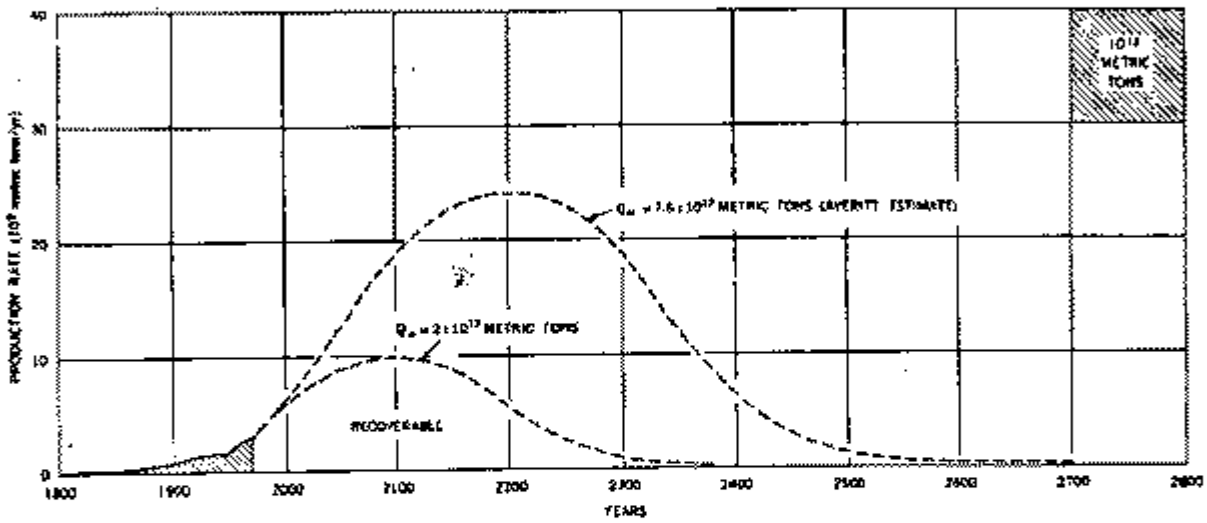
Fig 7. - Complete-cycle curves of world coal production for higher figure of 7.6 \times 10^{12} and lower figure of 2 \times 10^{12} metric tons for ultimate production (Hubbert, 1974a, fig. 21).
